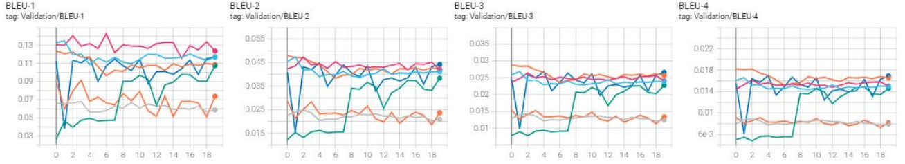
Figure 4: BLEU scores for second experiment
