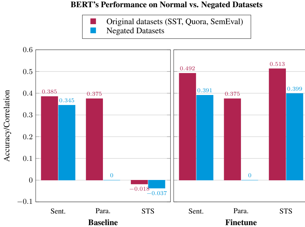
Figure 1: Side-by-side graphs comparing accuracy/correlation scores of the three tasks between original and negated datasets.
