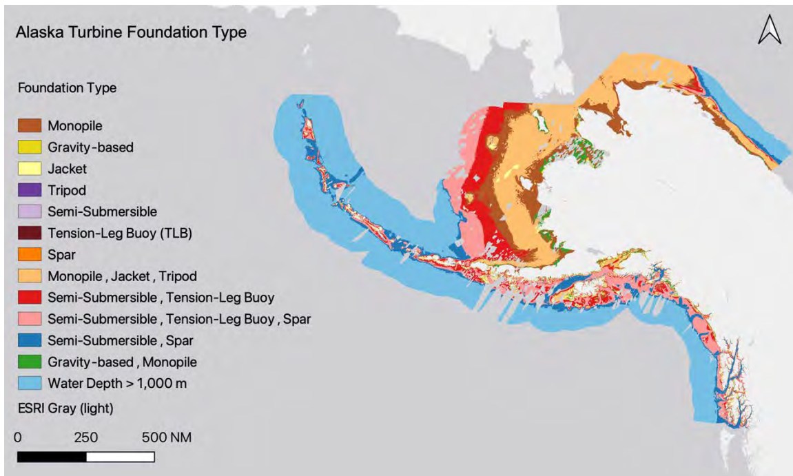
Figure S7.5: Alaska Turbine Foundation Type colored by appropriate turbine foundation(s), determined according to water depth and seabed composition.
