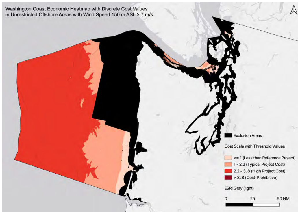
Figure S8.10: Washington Coast economic heatmap with discrete color ramp in relation to exclusion areas in black.
