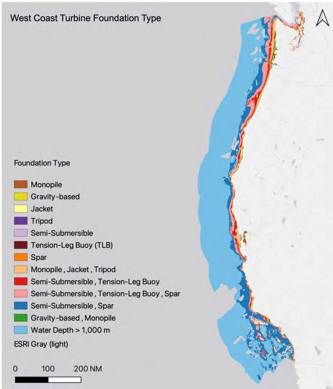
Figure S7.2: West Coast Turbine Foundation Type colored by appropriate turbine foundation(s), determined according to water depth and seabed composition.
