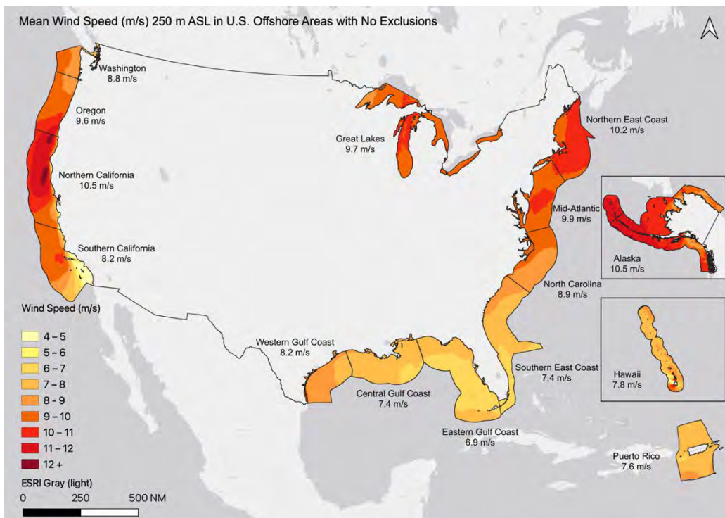
Figure S5.4: Mean wind speed (m/s) 250 m ASL in each region with no exclusions or wind speed restrictions. The color scale represents wind speed values between 4-12 m/s.
