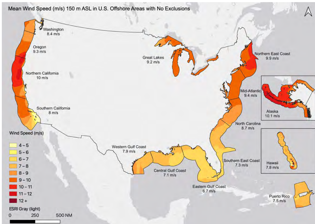
Figure S5.2: Mean wind speed (m/s) 150 m ASL in each region with no exclusions or wind speed restrictions. The color scale represents wind speed values between 4-12 m/s.
