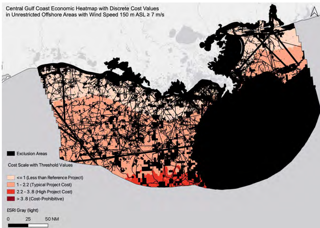
Figure S8.20: Central Gulf Coast economic heatmap with discrete color ramp in relation to exclusion areas in black.
