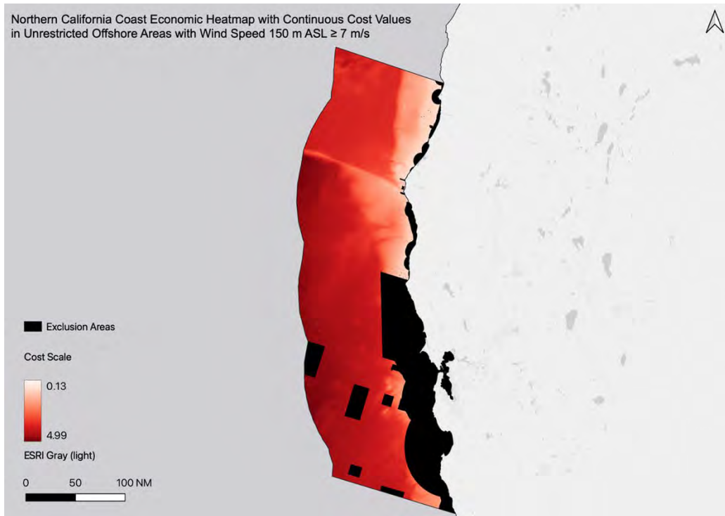
Figure S8.13: Northern California Coast economic heatmap with continuous color ramp in relation to exclusion areas in black. The unitless cost scale is the cost of a project relative to that of a reference project that accounts for water depth, transmission and port proximity, and wage rates of a typical coastal state. See Methods Section S5 for details.
