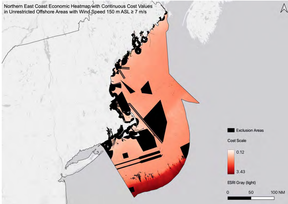
Figure S8.1: Northern East Coast economic heatmap with continuous color ramp in relation to exclusion areas in black. The unitless cost scale is the cost of a project relative to that of a reference project that accounts for water depth, transmission and port proximity, and wage rates of a typical coastal state. See Methods Section S5 for details.
