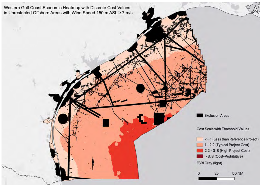
Figure S8.22: Western Gulf Coast economic heatmap with discrete color ramp in relation to exclusion areas in black.
