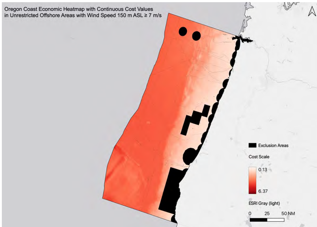
Figure S8.11: Oregon Coast economic heatmap with continuous color ramp in relation to exclusion areas in black. The unitless cost scale is the cost of a project relative to that of a reference project that accounts for water depth, transmission and port proximity, and wage rates of a typical coastal state. See Methods Section S5 for details.
