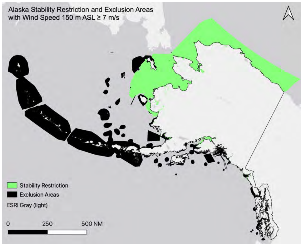
Figure S6.4: Alaska Stability Restriction (green) after accounting for all restrictions plus 150 m ASL \geq 7 m/s wind speed threshold (see Table S1 for details about each restriction layer). 1,398,720 km 2 (56.4%) of total Alaska area would be available for wind turbine development using a 30% stability threshold. There is a 27.6% difference in available area when restricting stability versus not.
