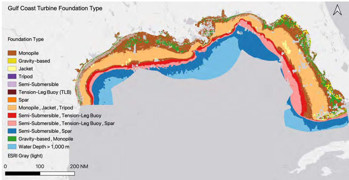
Figure S7.3: Gulf Coast Turbine Foundation Type colored by appropriate turbine foundation(s), determined according to water depth and seabed composition.
