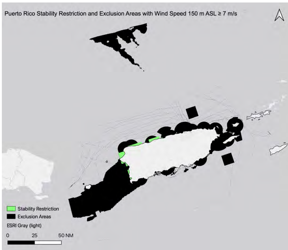
Figure S6.6: Puerto Rico Stability Restriction (green) after accounting for all restrictions plus 150 m ASL \geq 7 m/s wind speed threshold (see Table S1 for details about each restriction layer). 104,102 km 2 (88.6%) of total Puerto Rico area would be available for wind turbine development using a 30% stability threshold. There is a 0.053% difference in available area when restricting stability versus not.
