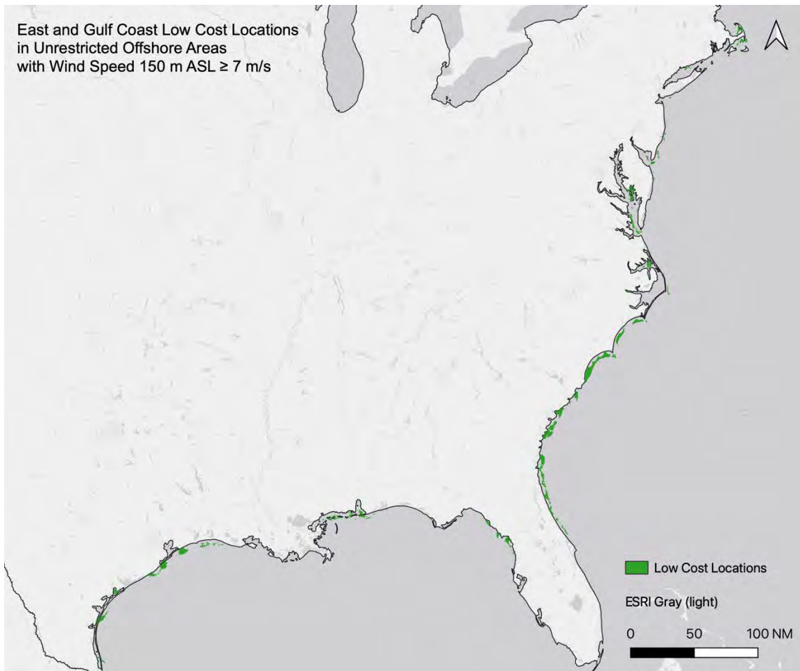
Figure S9.2: East and Gulf Coast Low Cost Locations (Scenario 2). A cost threshold of 0.68 was applied to exclude the Great Lakes. The areas shown in green can fulfill nearly the entire 30 GW by 2030 target set by the Biden Administration (very small areas on other coasts not shown) at the second lowest cost. In total 11,727 km 2 are required. Areas shown exclude restrictions and wind speeds below 7 m/s at 150 m ASL. Available capacity is calculated assuming uniform 7 m/s wind speed and capacity factor across all pixels to compute output power density.
