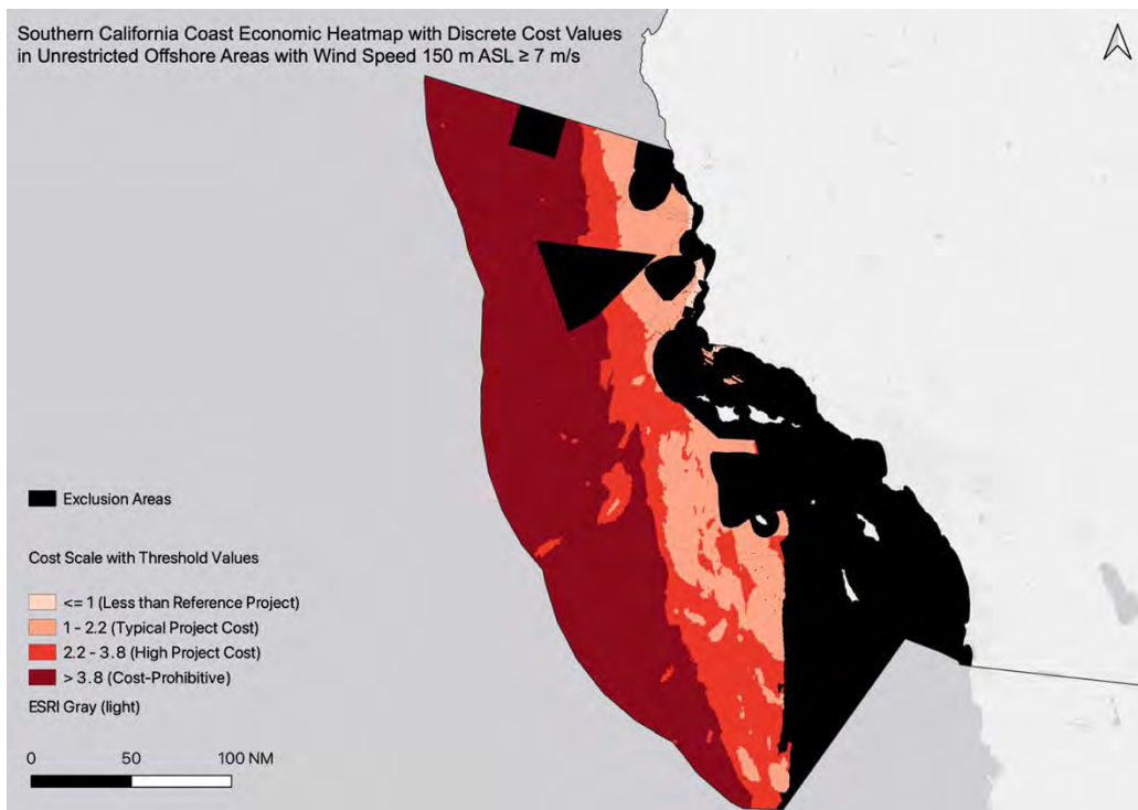
Figure S8.16: Southern California Coast economic heatmap with discrete color ramp in relation to exclusion areas in black.
