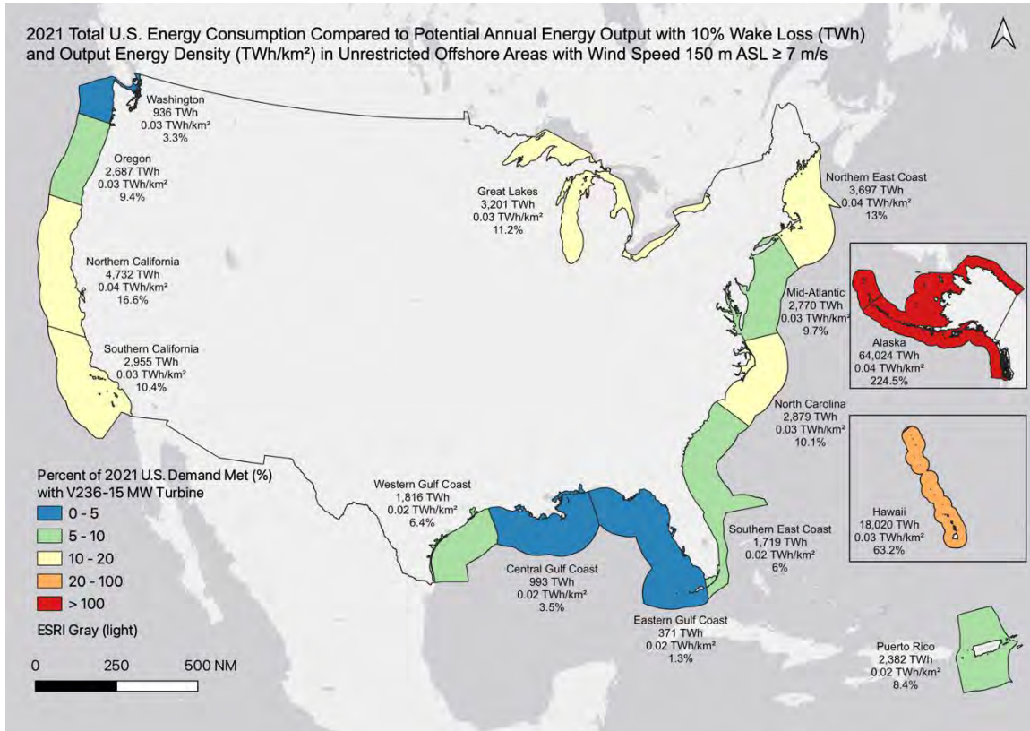
Figure S2.1: 2021 Total U.S. Energy Consumption Compared to Potential Annual Energy Output with 10% Wake Loss (TWh) and Output Energy Density (TWh/km 2 ). Regional potential energy output (TWh) (row 1) is divided by total U.S. all-purpose, end-use energy consumption across all sectors (commercial, residential, industrial, and transportation) in all 50 states, excluding Puerto Rico to compute Percent of 2021 U.S. Demand Met (%) (row 3). Also shown is output energy density (energy output divided by available area) (row 2). A wind speed threshold of 150 m ASL \geq 7 m/s and 10% (medium) wake loss scenario are used to compute each value. See Tables S11-14 for all combinations of hub height, wind speed thresholds, and wake loss scenarios.
