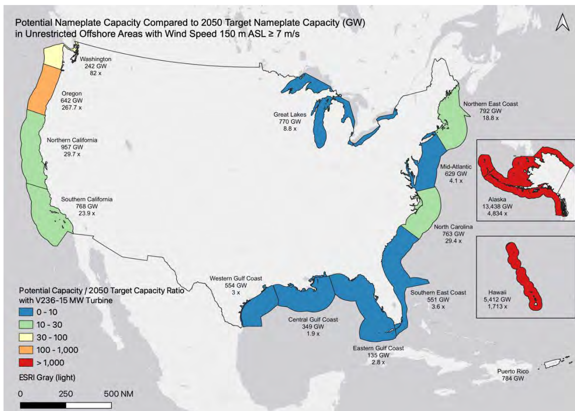
Figure S1.1: Potential Nameplate Capacity Compared to 2050 Target Nameplate Capacity (GW). Compares potential nameplate capacity (GW) in all unrestricted offshore areas (Table S1) calculated with V236-15 MW turbine and wind speed at 150 m ASL \geq 7 m/s (row 1) to 2050 total nameplate capacity (GW) needed needed to match power demand with supply, storage, and demand response continuously during 2050-2051, as calculated in Jacobson et. al. [104], presented as a ratio (row 2). See Figure S1.2 and Tables S6-7 for all combinations of hub heights and wind speed thresholds.
