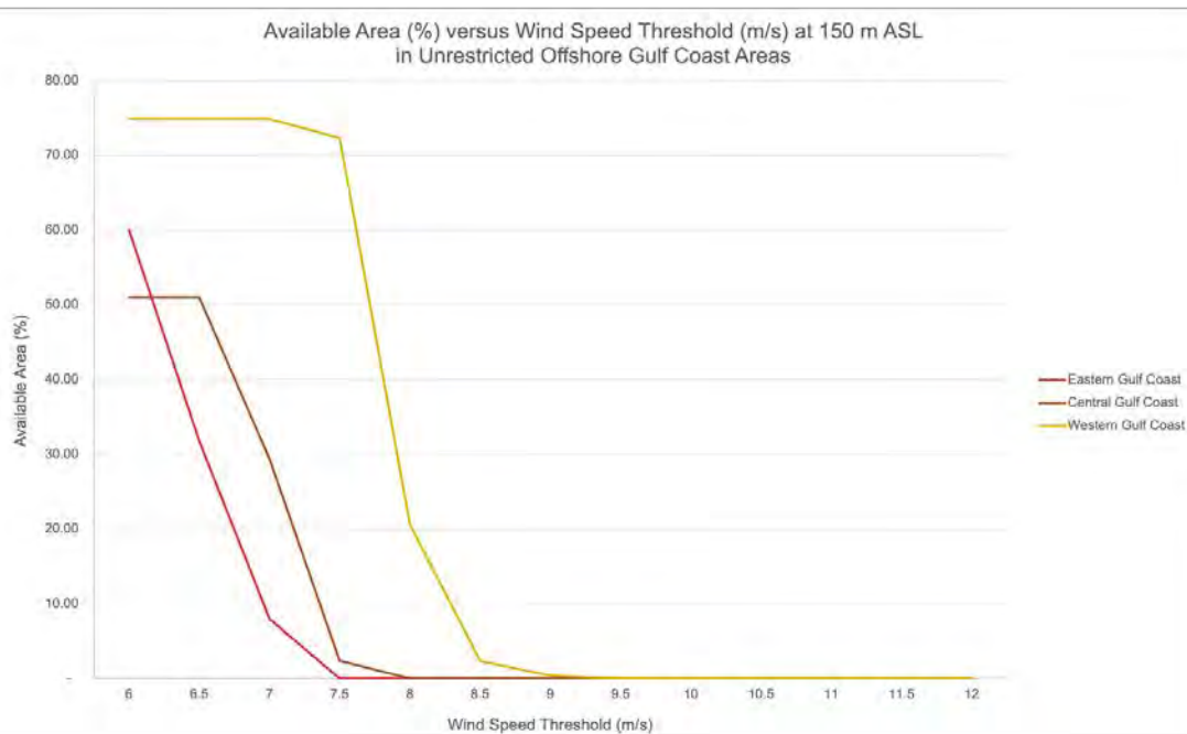
Figure S4.2: Available area (%) for each wind speed threshold (m/s) at 150 m ASL in each Gulf Coast region (Eastern Gulf Coast, Central Gulf Coast, and Western Gulf Coast), after taking into account all restrictions in Table S1.
