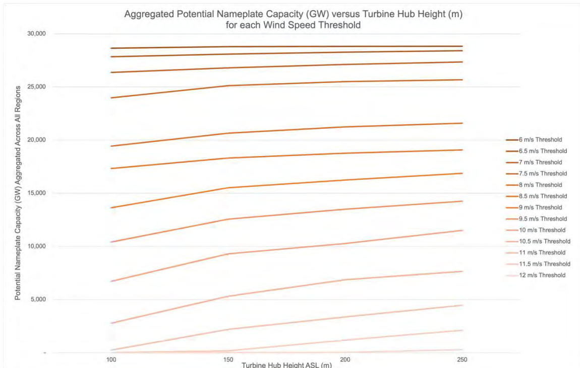
Figure S1.2: Aggregated Potential Nameplate Capacity (GW) versus Turbine Hub Height (m). See Tables S6-7 for a breakdown of potential nameplate capacity for each wind speed threshold and hub height scenario by region.
