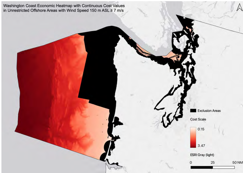
Figure S8.9: Washington Coast economic heatmap with continuous color ramp in relation to exclusion areas in black. The unitless cost scale is the cost of a project relative to that of a reference project that accounts for water depth, transmission and port proximity, and wage rates of a typical coastal state. See Methods Section S5 for details.
