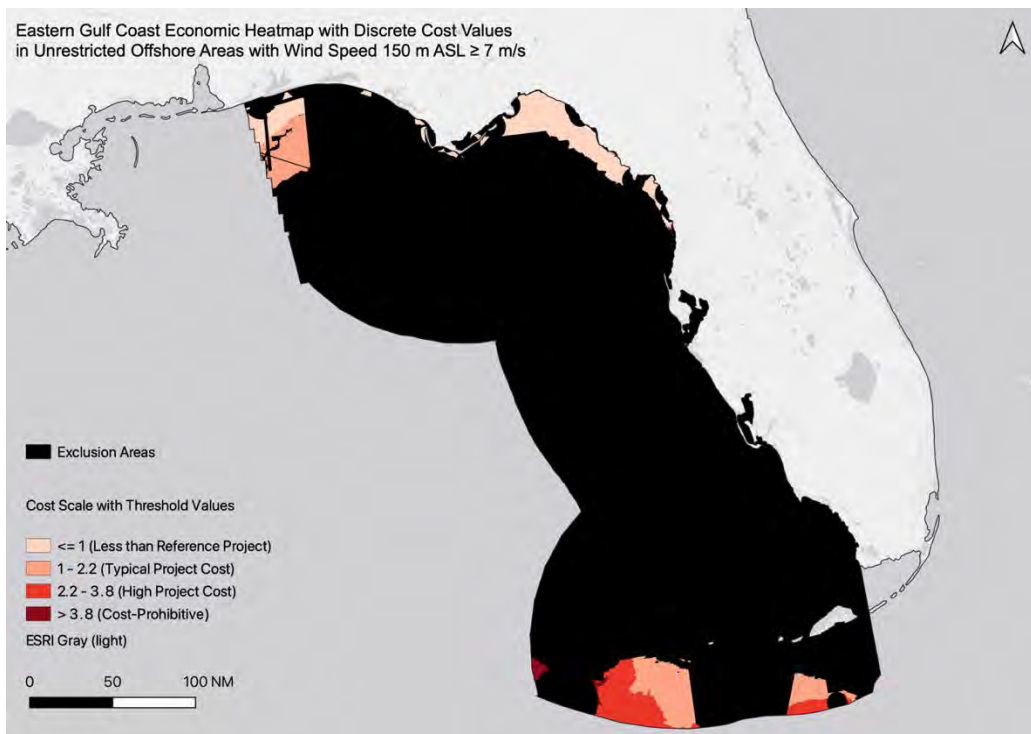
Figure S8.18: Eastern Gulf Coast economic heatmap with discrete color ramp in relation to exclusion areas in black.
