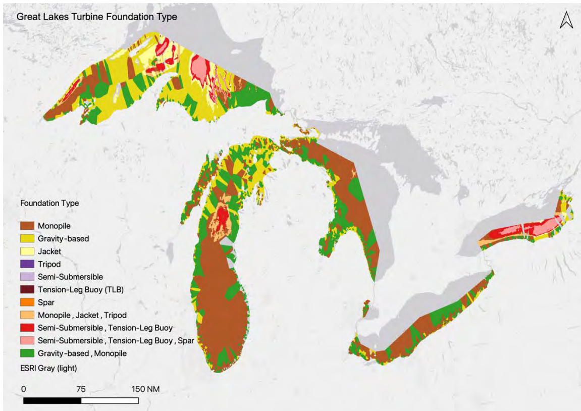
Figure S7.4: Great Lakes Turbine Foundation Type colored by appropriate turbine foundation(s), determined according to water depth and seabed composition.
