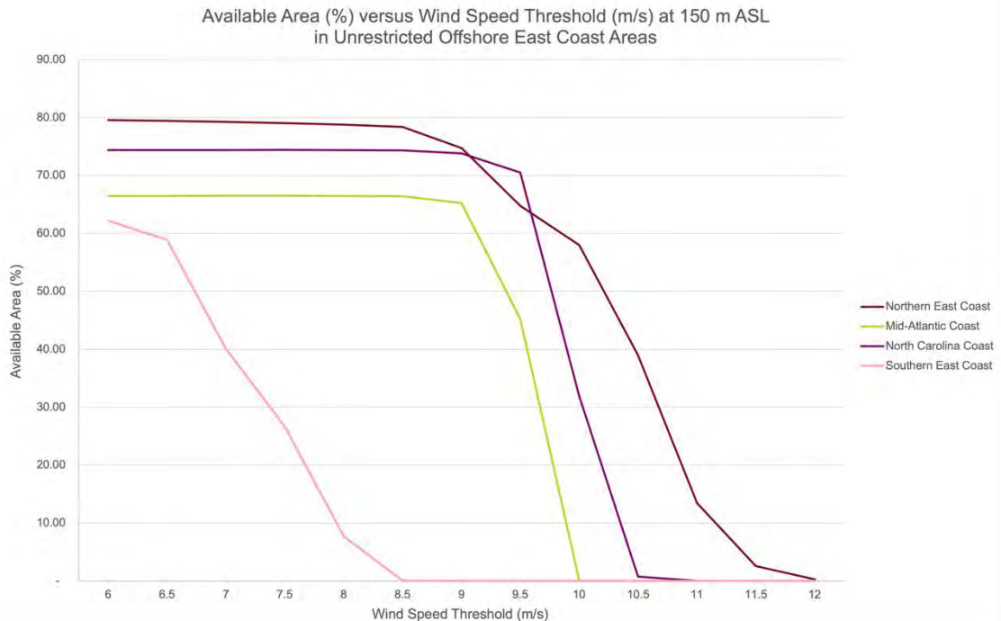
Figure S4.1: Available area (%) for each wind speed threshold (m/s) at 150 m ASL in each East Coast region (Northern East Coast, Mid-Atlantic Coast, North Carolina Coast, and Southern East Coast), after taking into account all restrictions in Table S1.
