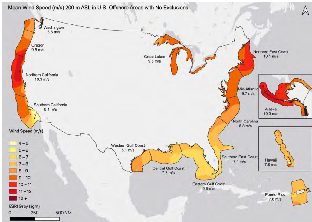
Figure S5.3: Mean wind speed (m/s) 200 m ASL in each region with no exclusions or wind speed restrictions. The color scale represents wind speed values between 4-12 m/s.
