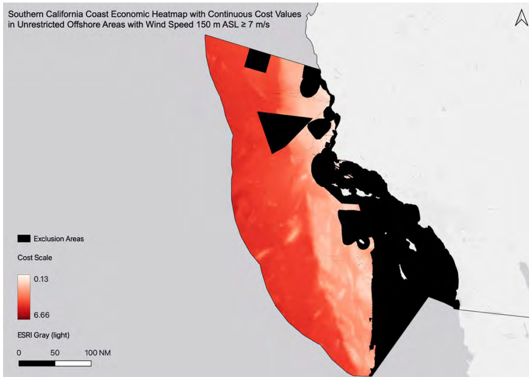
Figure S8.15: Southern California Coast economic heatmap with continuous color ramp in relation to exclusion areas in black. The unitless cost scale is the cost of a project relative to that of a reference project that accounts for water depth, transmission and port proximity, and wage rates of a typical coastal state. See Methods Section S5 for details.
