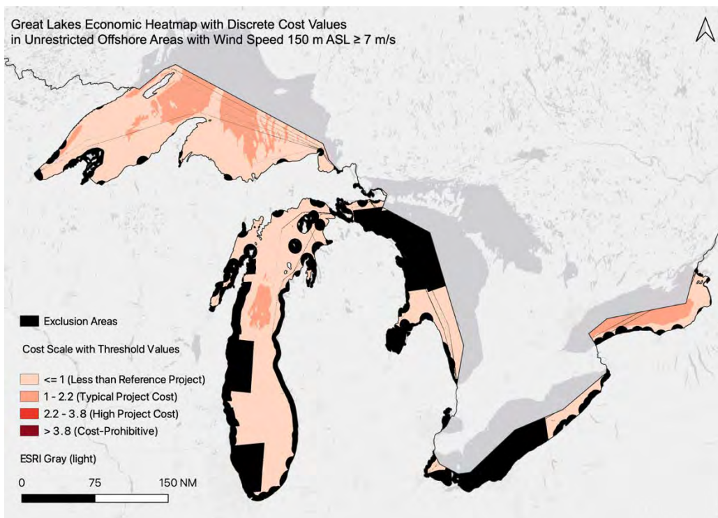
Figure S8.24: Great Lakes economic heatmap with discrete color ramp in relation to exclusion areas in black.
