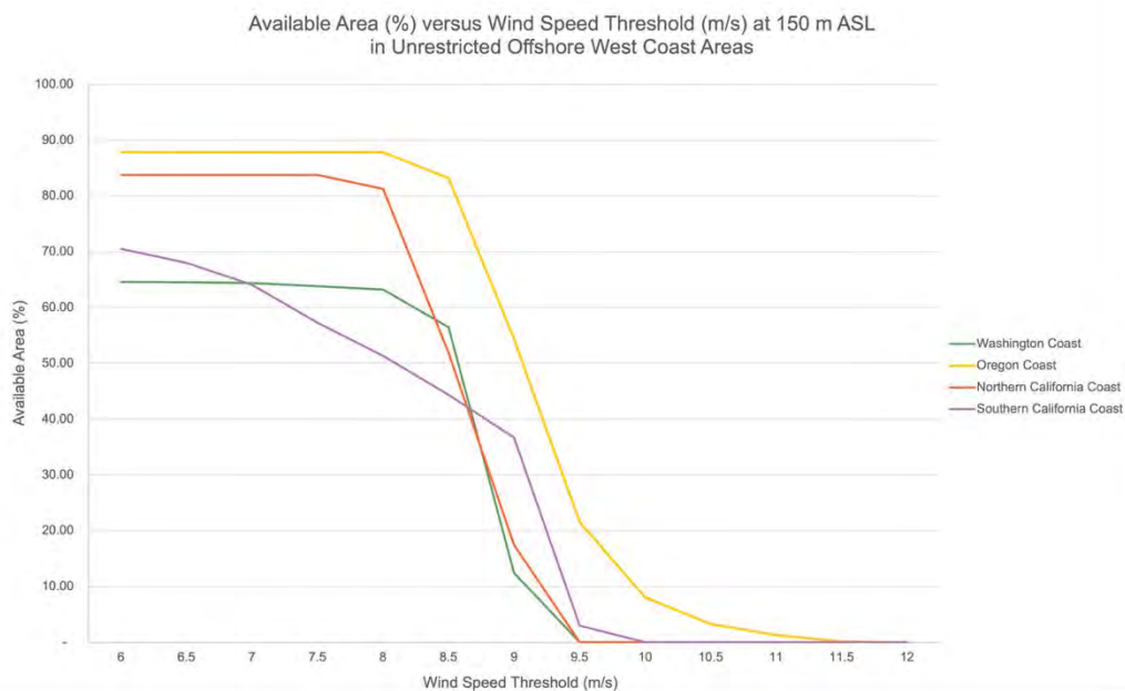
Figure S4.3: Available area (%) for each wind speed threshold (m/s) at 150 m ASL in each West Coast region (Washington Coast, Oregon Coast, Northern California Coast, and Southern California Coast), after taking into account all restrictions in Table S1.
