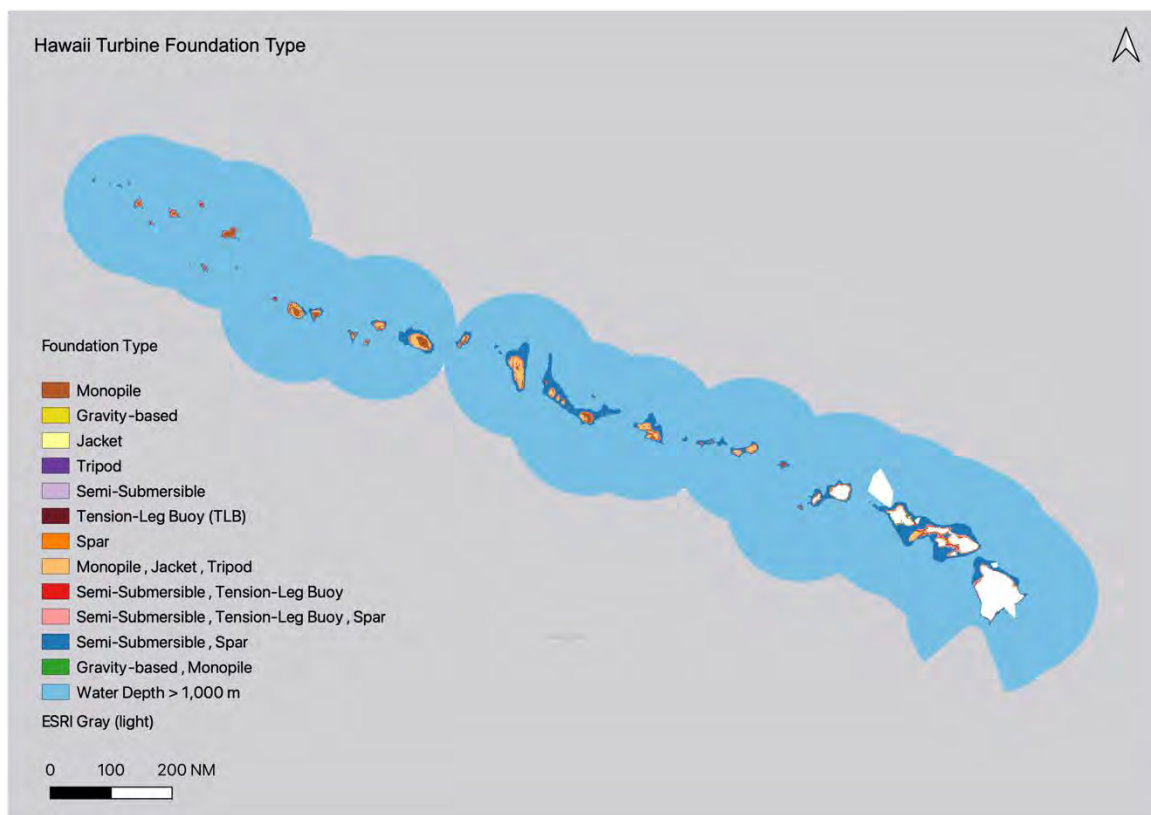
Figure S7.6: Hawaii Turbine Foundation Type colored by appropriate turbine foundation(s), determined according to water depth and seabed composition.
