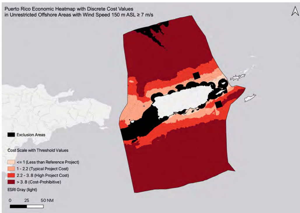
Figure S8.30: Puerto Rico economic heatmap with discrete color ramp in relation to exclusion areas in black.
