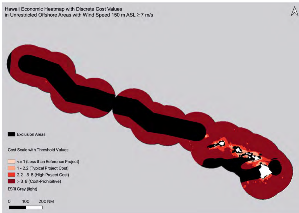
Figure S8.28: Hawaii economic heatmap with discrete color ramp in relation to exclusion areas in black.
