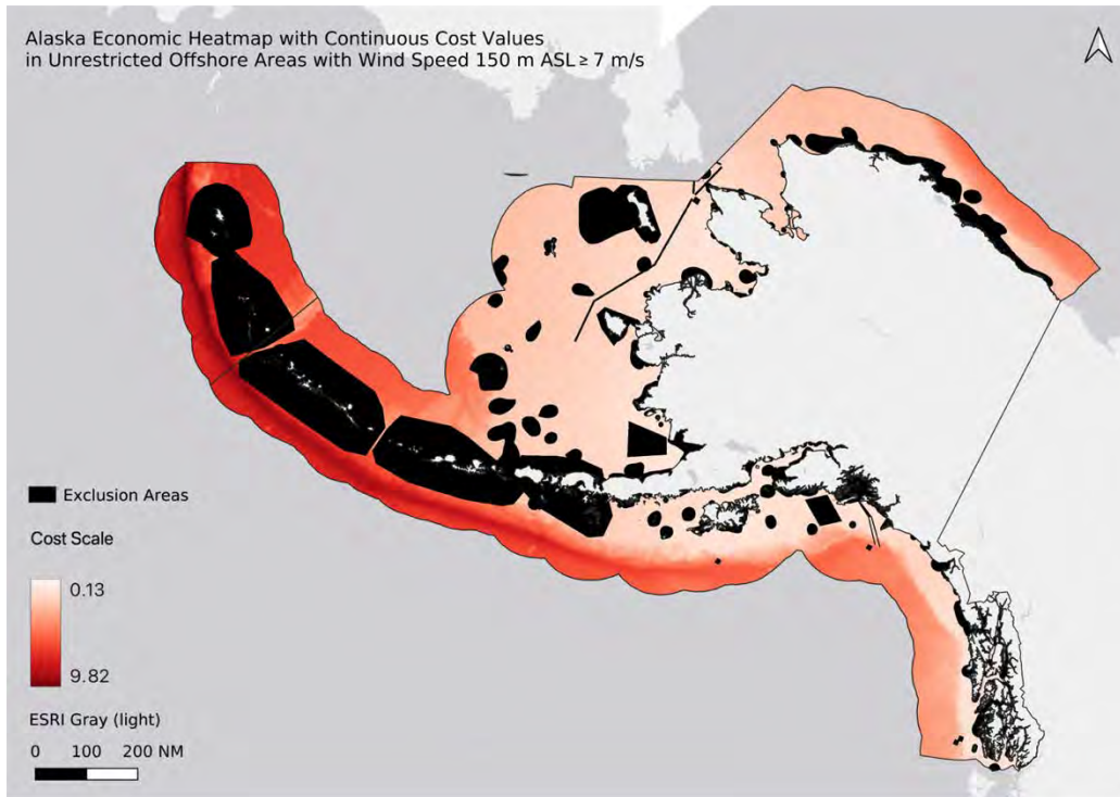
Figure S8.25: Alaska economic heatmap with continuous color ramp in relation to exclusion areas in black. The unitless cost scale is the cost of a project relative to that of a reference project that accounts for water depth, transmission and port proximity, and wage rates of a typical coastal state. See Methods Section S5 for details.
