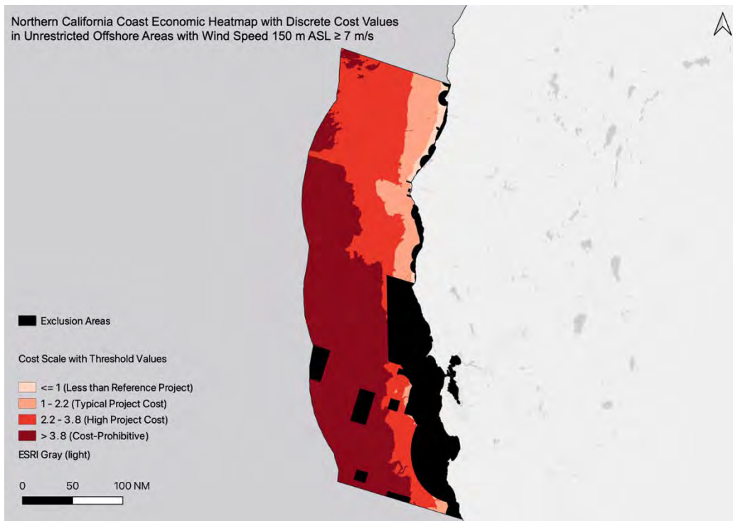
Figure S8.14: Northern California Coast economic heatmap with discrete color ramp in relation to exclusion areas in black.
