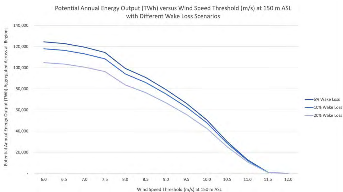
Figure S2.2: Potential Annual Energy Output (TWh) versus Wind Speed Threshold (m/s). Graph shows how cumulative energy output at 150 m ASL varies with wind speed thresholds for different wake loss scenarios (dark blue: 5%, medium blue: 10%, light blue: 20%). Not shown is no wake loss scenario. See Tables S11-12 for all hub height and wake loss combinations.
