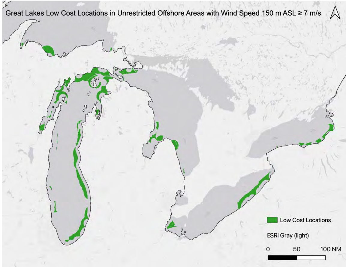
Figure S9.1: Great Lakes Low Cost Locations (Scenario 1). The areas shown in green can fulfill nearly the entire 30 GW by 2030 target set by the Biden Administration (very small areas on other coasts not shown) at the lowest cost. In total 11,727 km 2 are required. Areas shown exclude restrictions and wind speeds below 7 m/s at 150 m ASL. Available capacity is calculated assuming uniform 7 m/s wind speed and capacity factor across all pixels to compute output power density.
