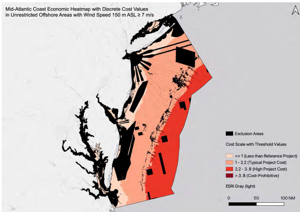
Figure S8.4: Mid-Atlantic Coast economic heatmap with discrete color ramp in relation to exclusion areas in black.
