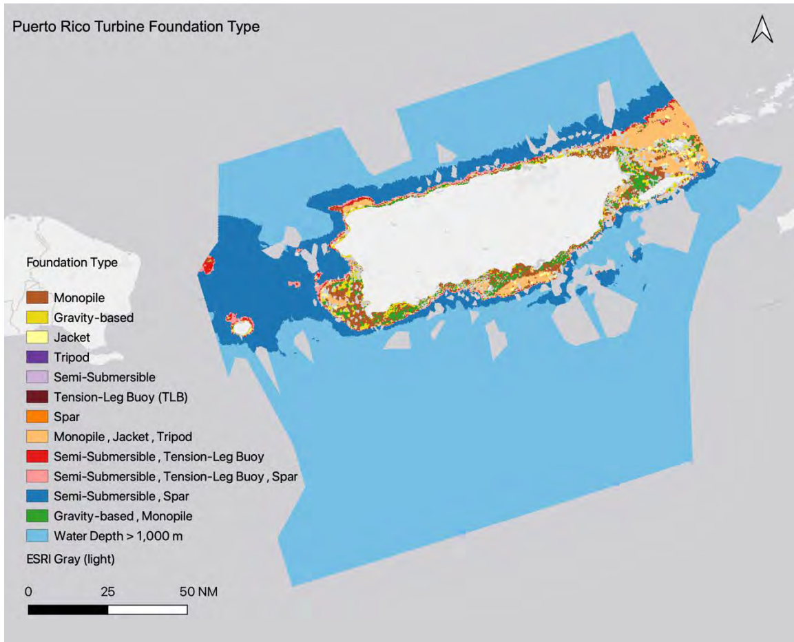
Figure S7.7: Puerto Rico Turbine Foundation Type colored by appropriate turbine foundation(s), determined according to water depth and seabed composition.
