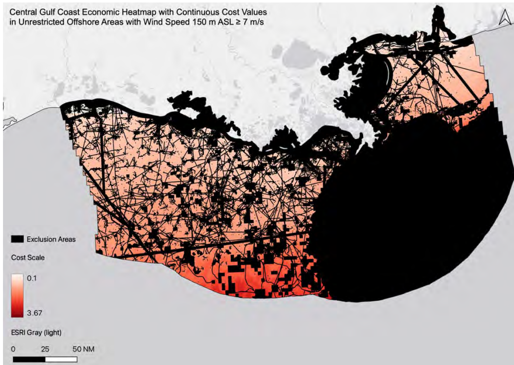
Figure S8.19: Central Gulf Coast economic heatmap with continuous color ramp in relation to exclusion areas in black. The unitless cost scale is the cost of a project relative to that of a reference project that accounts for water depth, transmission and port proximity, and wage rates of a typical coastal state. See Methods Section S5 for details.
