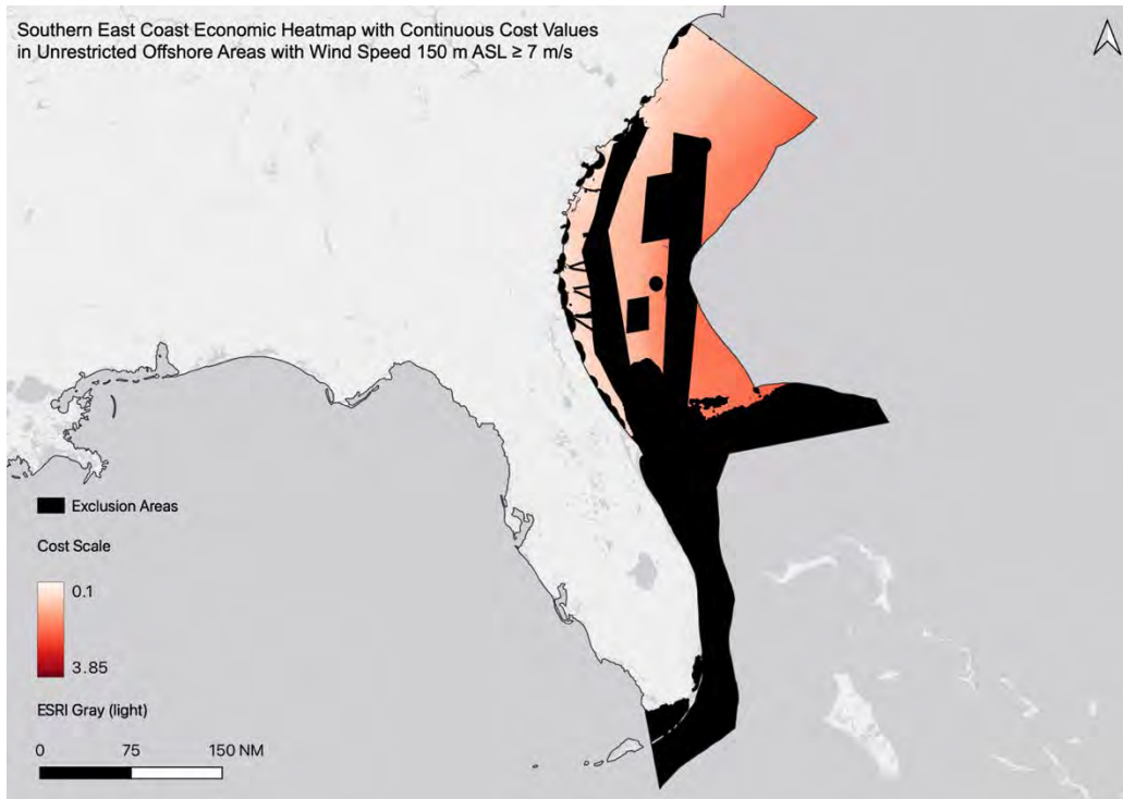
Figure S8.7: Southern East Coast economic heatmap with continuous color ramp in relation to exclusion areas in black. The unitless cost scale is the cost of a project relative to that of a reference project that accounts for water depth, transmission and port proximity, and wage rates of a typical coastal state. See Methods Section S5 for details.
