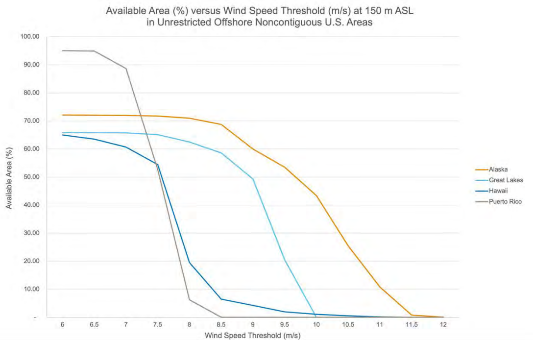
Figure S4.4: Available area (%) for each wind speed threshold (m/s) at 150 m ASL in each noncontiguous U.S. region (Alaska, Great Lakes, Hawaii, and Puerto Rico), after taking into account all restrictions in Table S1.
