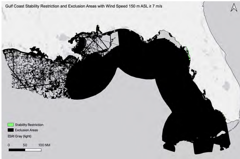
Figure S6.3: Gulf Coast Stability Restriction (green) after accounting for all restrictions plus 150 m ASL \geq 7 m/s wind speed threshold (see Table S1 for details about each restriction layer). 137,675 km 2 (28.6%) of total Gulf Coast area would be available for wind turbine development using a 30% stability threshold. There is a 0.09% difference in available area when restricting stability versus not.
