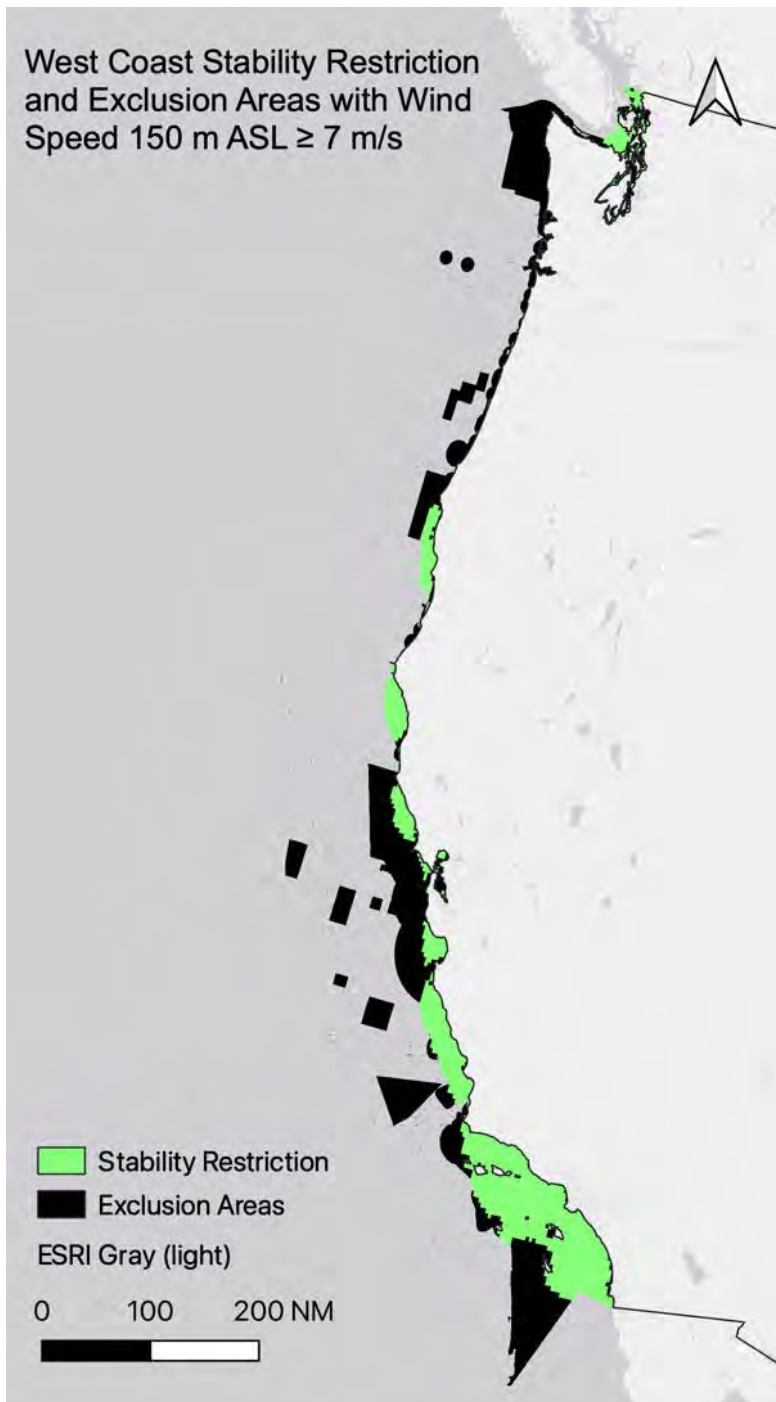
Figure S6.2: West Coast Stability Restriction (green) after accounting for all restrictions plus 150 m ASL \geq 7 m/s wind speed threshold (see Table S1 for details about each restriction layer). 339,791 km 2 (72.8%) of total West Coast area would be available for wind turbine development using a 30% stability threshold. Off the coast of Southern California, stability accounts for much of the excluded area, but other restrictions layered underneath already excluded the area, so the percent difference between the two scenarios is not great (2.8% difference between stability restricted versus not).
