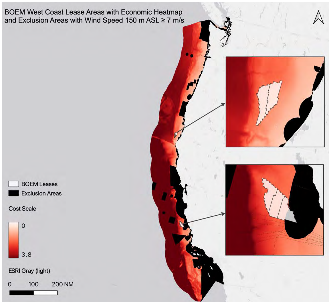
Figure S3.2: BOEM West Coast Lease Areas with Economic Heatmap and Exclusion Areas.
