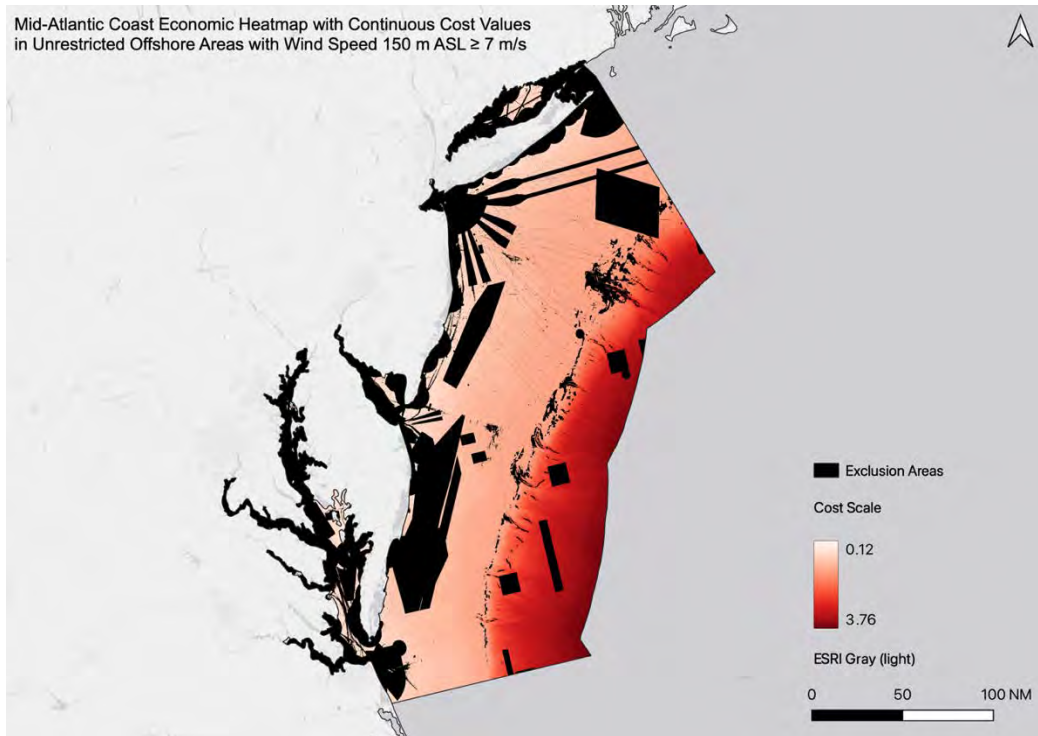
Figure S8.3: Mid-Atlantic Coast economic heatmap with continuous color ramp in relation to exclusion areas in black. The unitless cost scale is the cost of a project relative to that of a reference project that accounts for water depth, transmission and port proximity, and wage rates of a typical coastal state. See Methods Section S5 for details.
